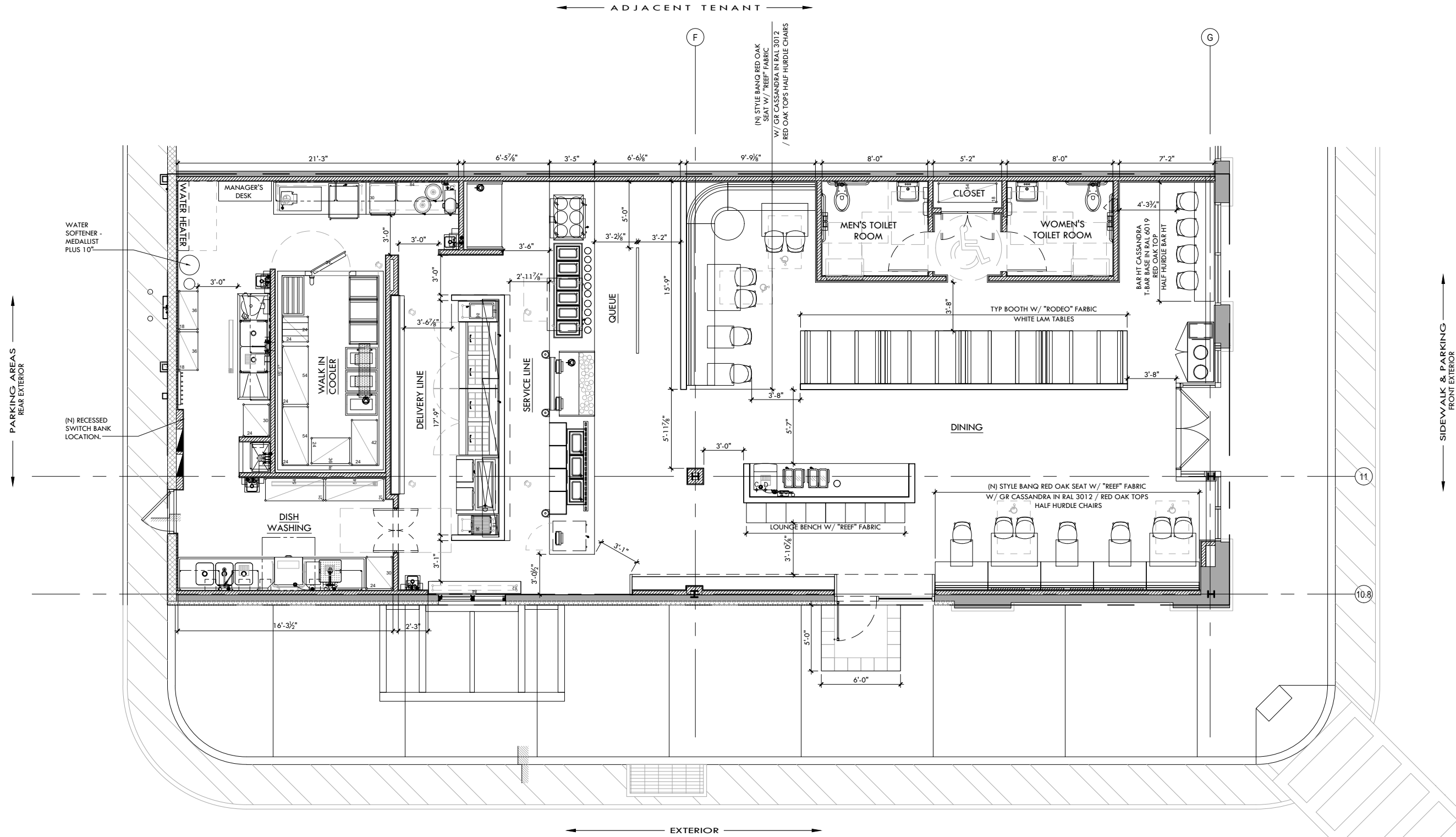
1 DD PROPOSED FIXTURE PLAN
